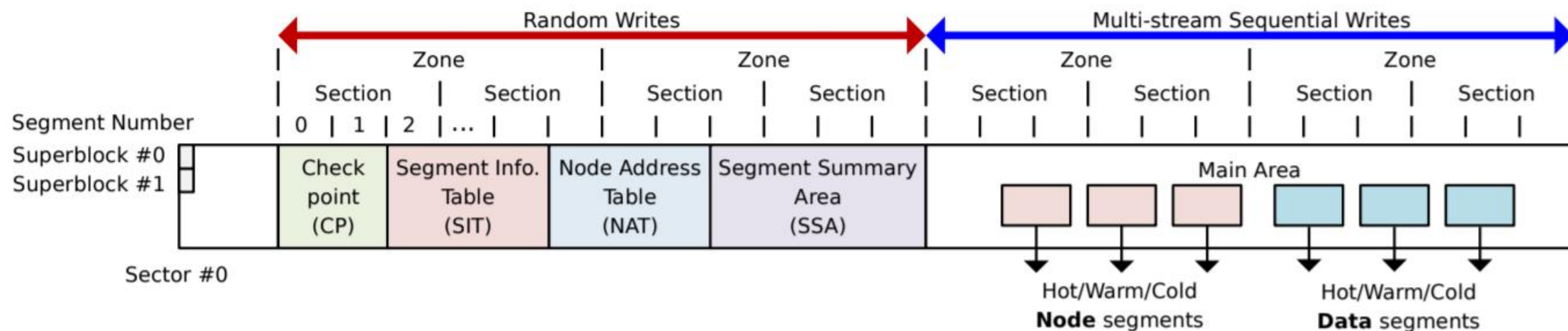
Figure 1: On-disk layout of F2FS.
